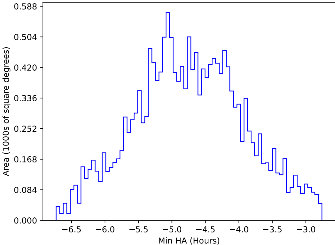
extra_ss_neo4_v3.4_10yrs WFD all bands: Min HA
