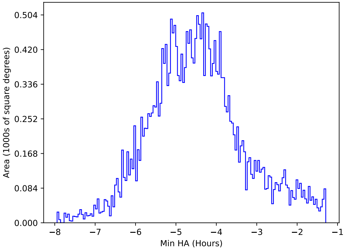
extra_ss_neo4_v3.4_10yrs All sky all bands: Min HA
