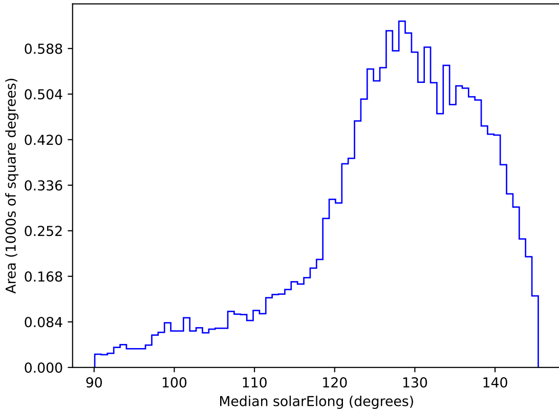
extra_ss_neo4_v3.4_10yrs WFD z band: Median solarElong
