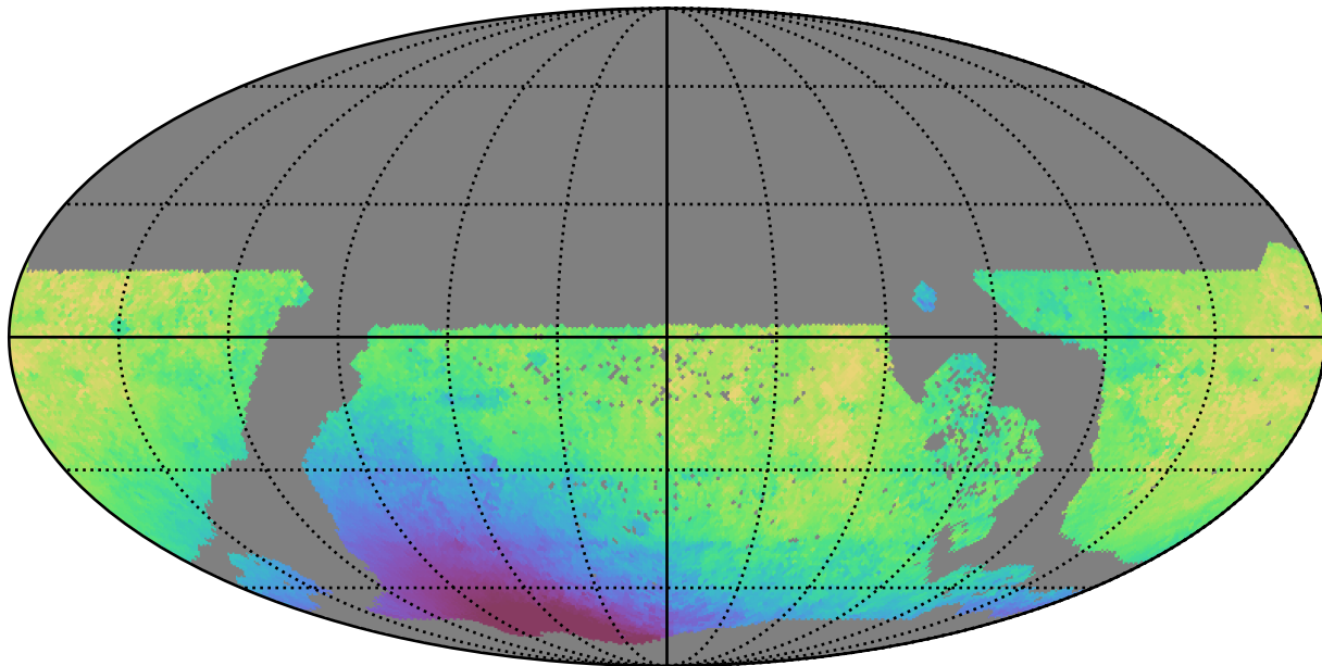
extra_ss_neo4_v3.4_10yrs WFD y band: Median solarElong
