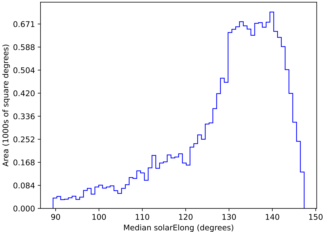
extra_ss_neo4_v3.4_10yrs WFD y band: Median solarElong
