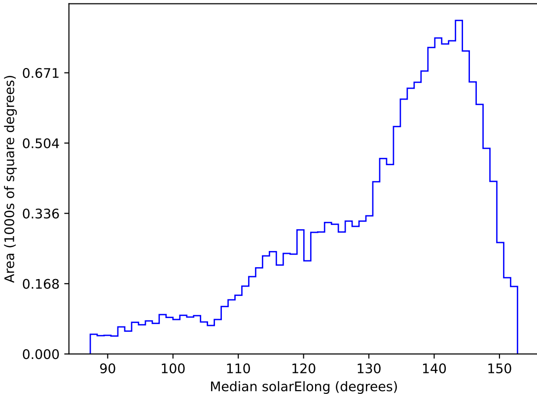
extra_ss_neo4_v3.4_10yrs WFD u band: Median solarElong
