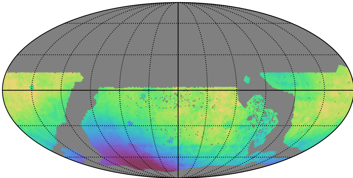
extra_ss_neo4_v3.4_10yrs WFD r band: Median solarElong
