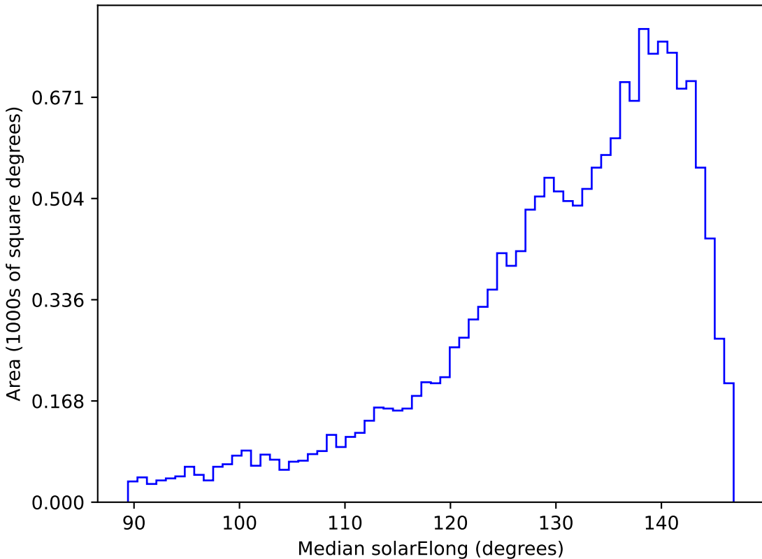
extra_ss_neo4_v3.4_10yrs WFD r band: Median solarElong
