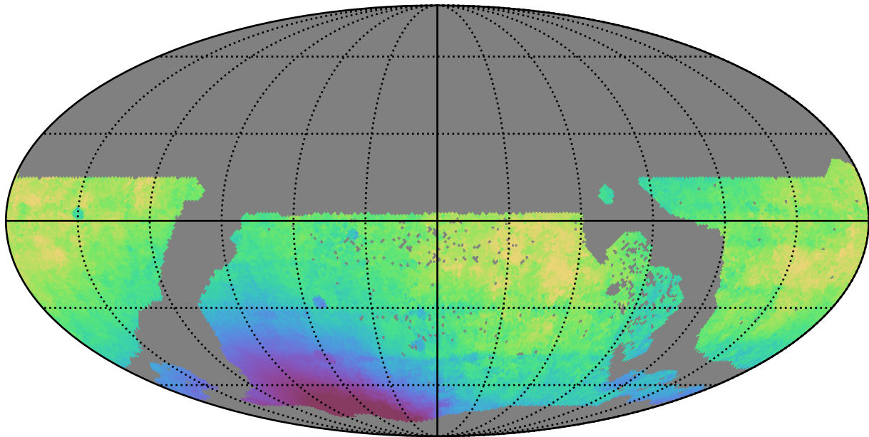
extra_ss_neo4_v3.4_10yrs WFD i band: Median solarElong
