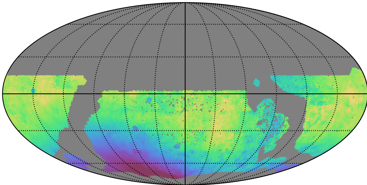
extra_ss_neo4_v3.4_10yrs WFD g band: Median solarElong
