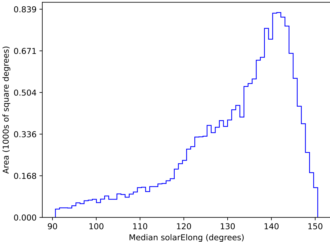
extra_ss_neo4_v3.4_10yrs WFD g band: Median solarElong
