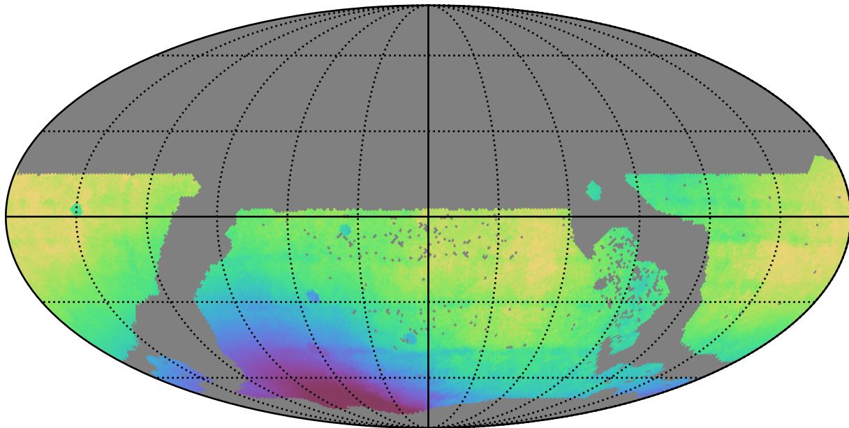
extra_ss_neo4_v3.4_10yrs WFD all bands: Median solarElong
