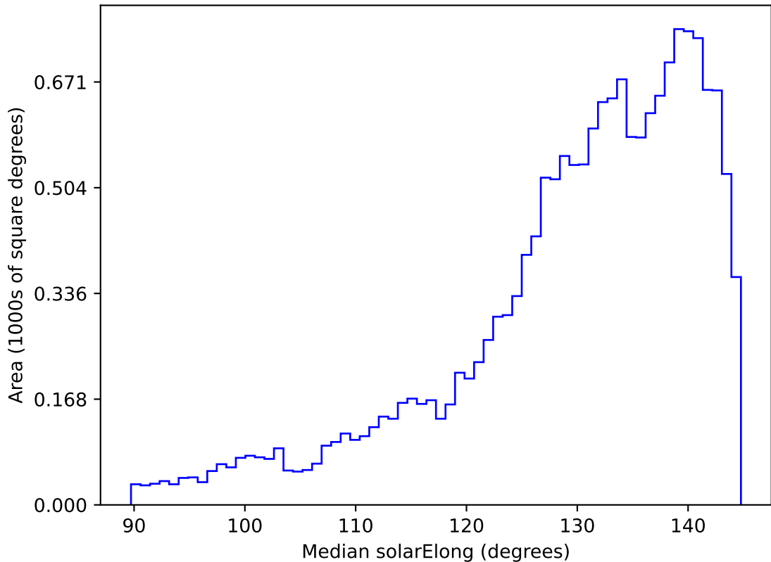
extra_ss_neo4_v3.4_10yrs WFD all bands: Median solarElong
