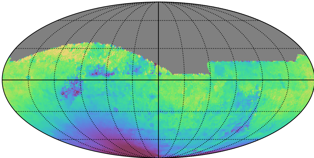
extra_ss_neo4_v3.4_10yrs All sky z band: Median solarElong
