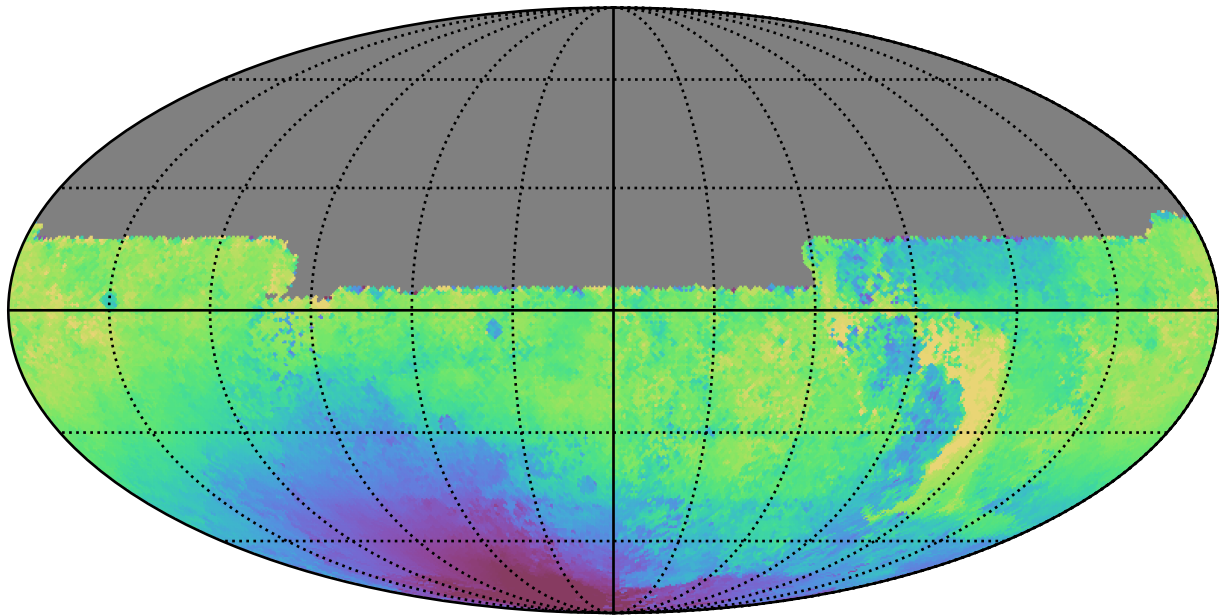
extra_ss_neo4_v3.4_10yrs All sky u band: Median solarElong
