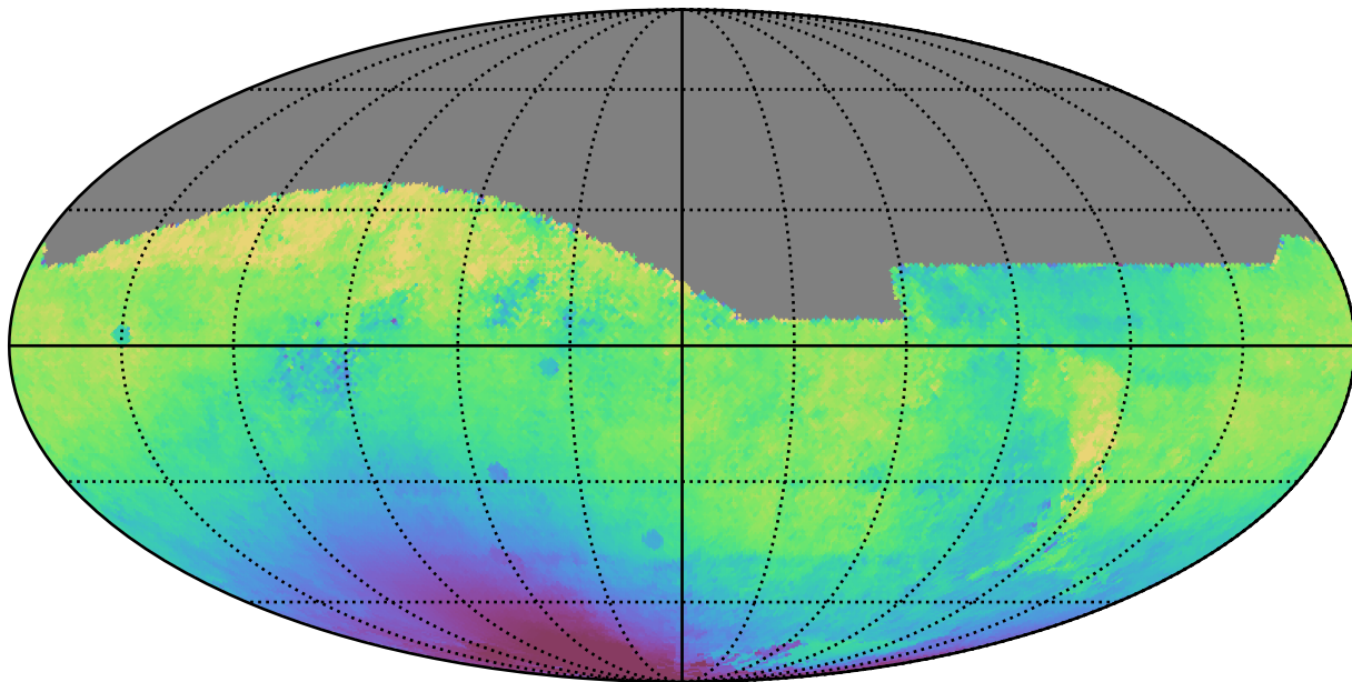
extra_ss_neo4_v3.4_10yrs All sky r band: Median solarElong
