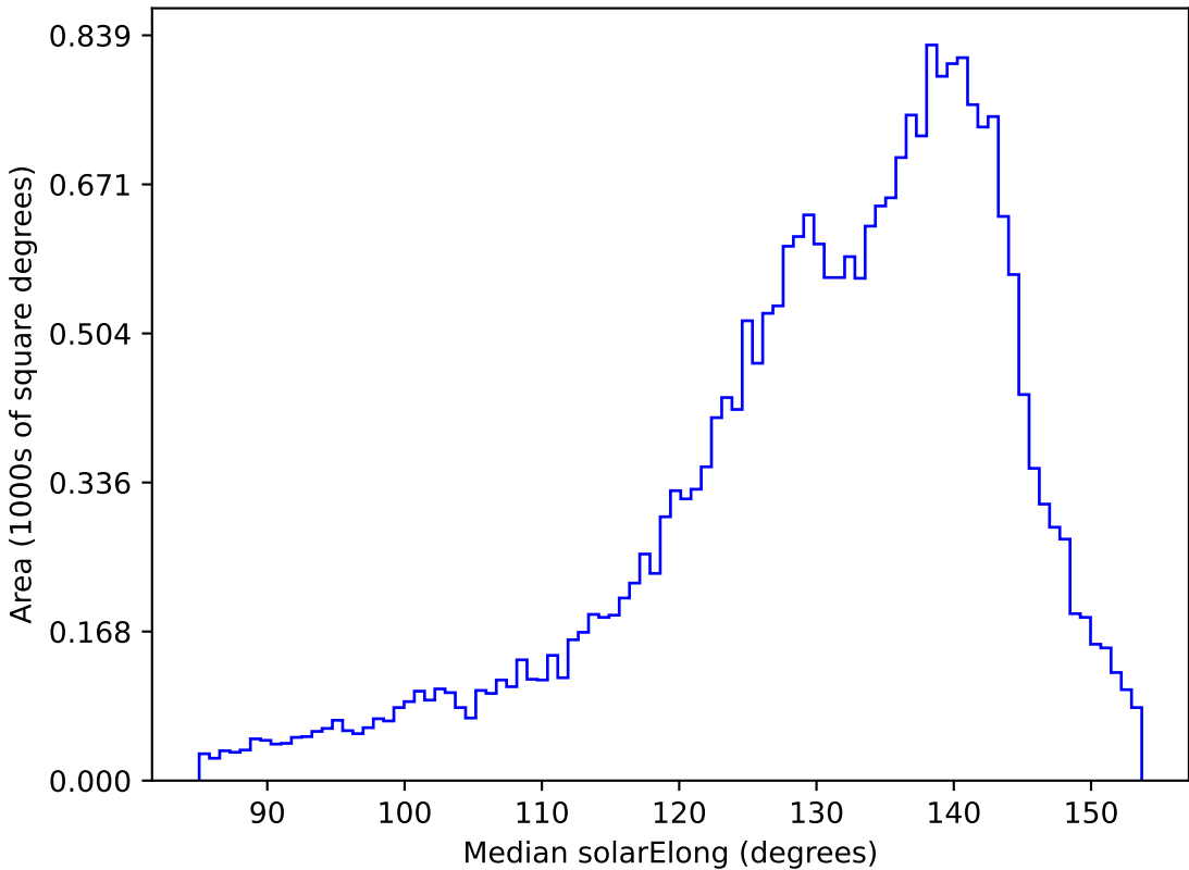
extra_ss_neo4_v3.4_10yrs All sky r band: Median solarElong
