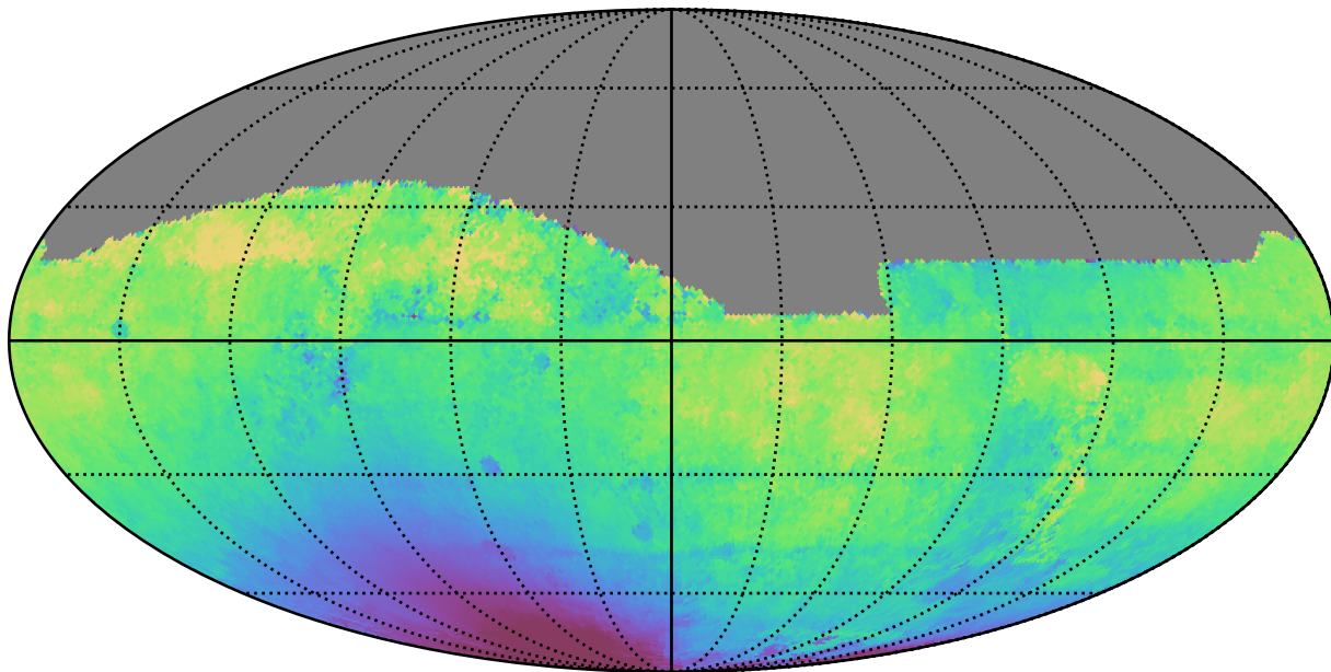
extra_ss_neo4_v3.4_10yrs All sky i band: Median solarElong
