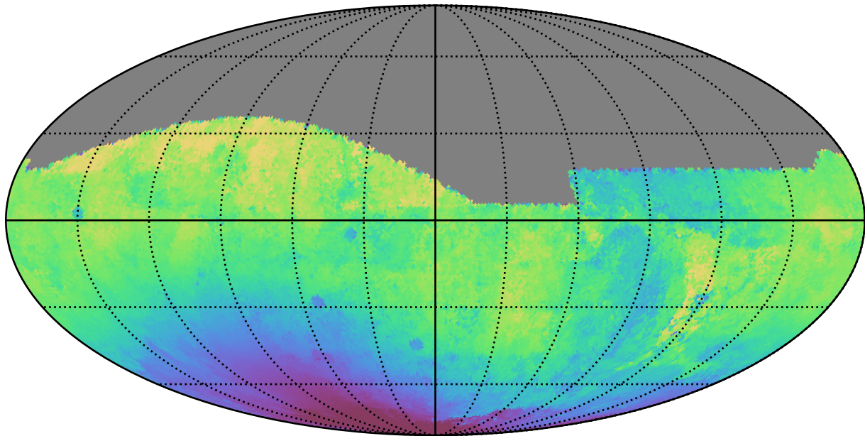
extra_ss_neo4_v3.4_10yrs All sky g band: Median solarElong
