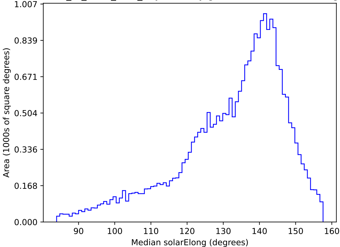
extra_ss_neo4_v3.4_10yrs All sky g band: Median solarElong
