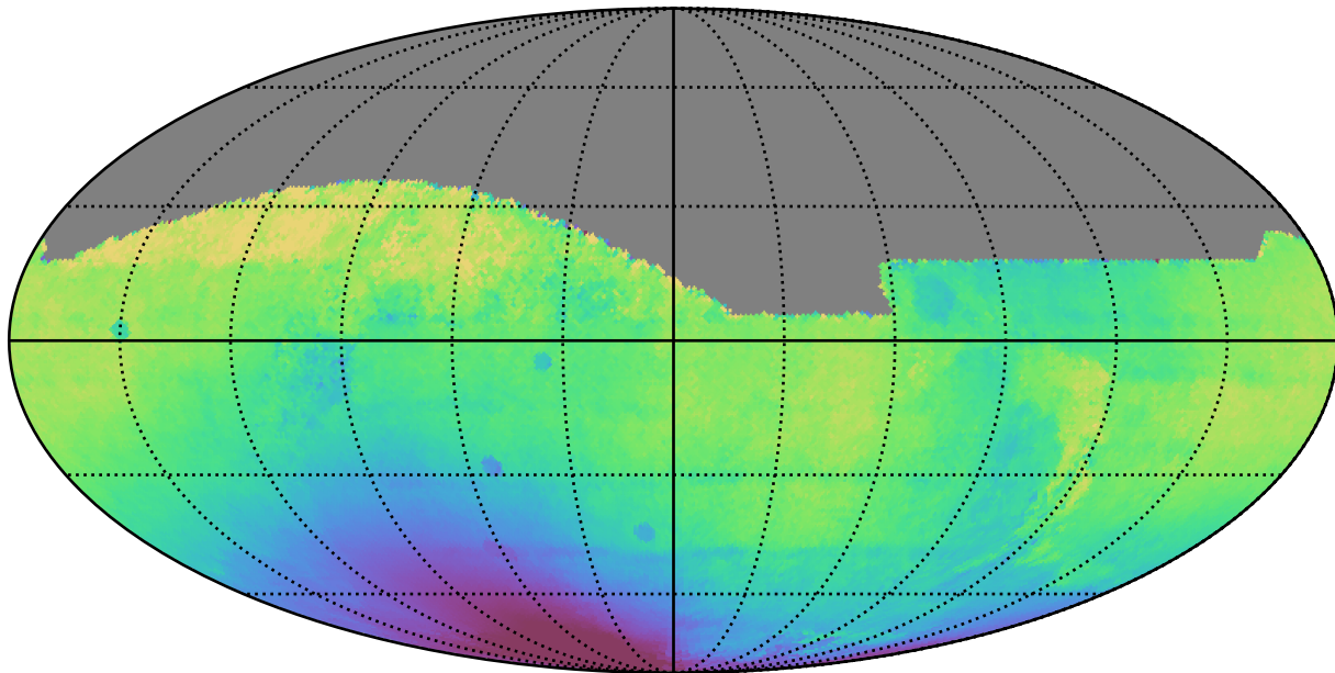
extra_ss_neo4_v3.4_10yrs All sky all bands: Median solarElong
