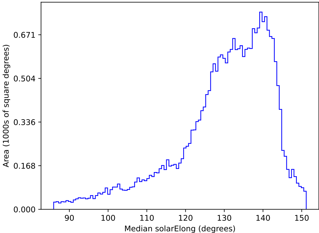
extra_ss_neo4_v3.4_10yrs All sky all bands: Median solarElong
