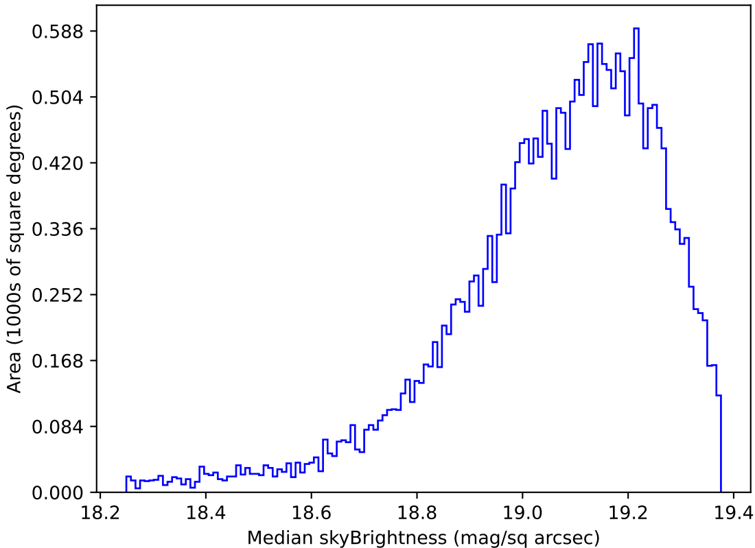
extra_ss_neo4_v3.4_10yrs Yr 1 z band: Median skyBrightness
