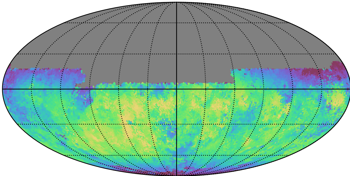
extra_ss_neo4_v3.4_10yrs Yr 1 y band: Median skyBrightness
