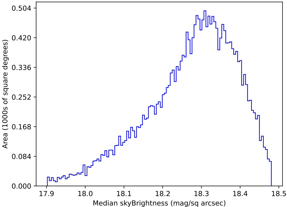
extra_ss_neo4_v3.4_10yrs Yr 1 y band: Median skyBrightness
