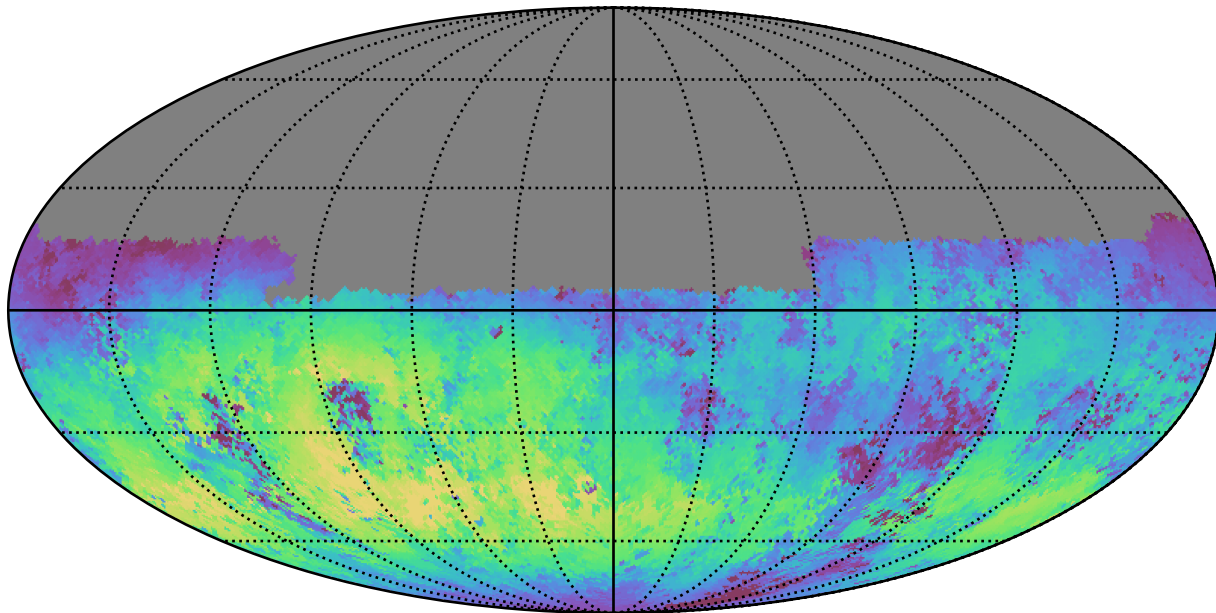
extra_ss_neo4_v3.4_10yrs Yr 1 u band: Median skyBrightness
