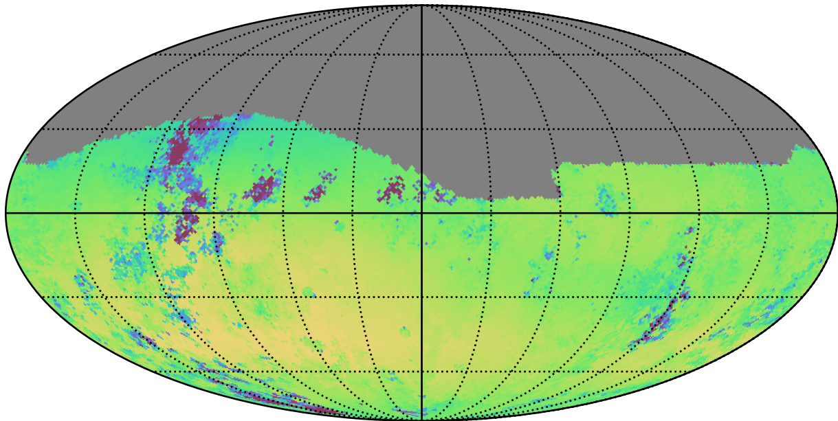
extra_ss_neo4_v3.4_10yrs Yr 1 r band: Median skyBrightness
