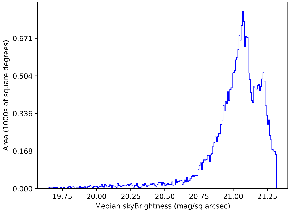
extra_ss_neo4_v3.4_10yrs Yr 1 r band: Median skyBrightness
