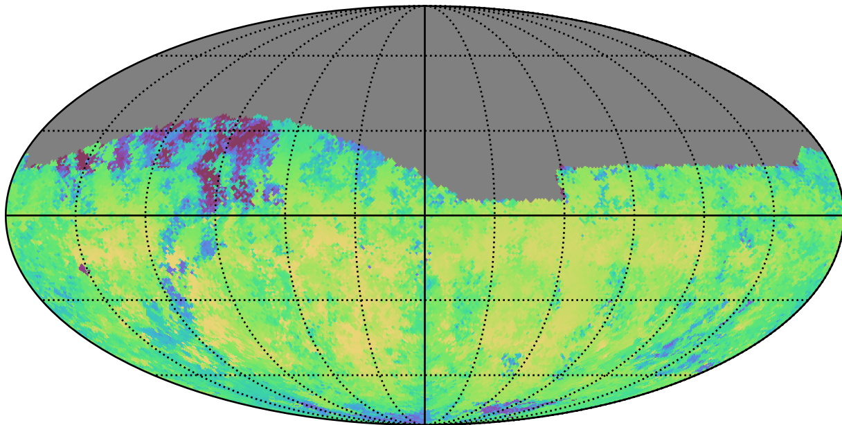
extra_ss_neo4_v3.4_10yrs Yr 1 i band: Median skyBrightness
