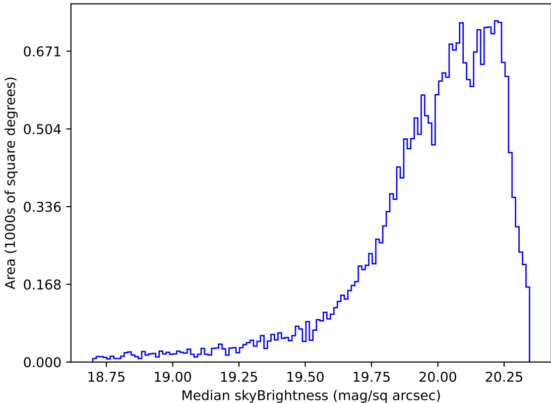
extra_ss_neo4_v3.4_10yrs Yr 1 i band: Median skyBrightness
