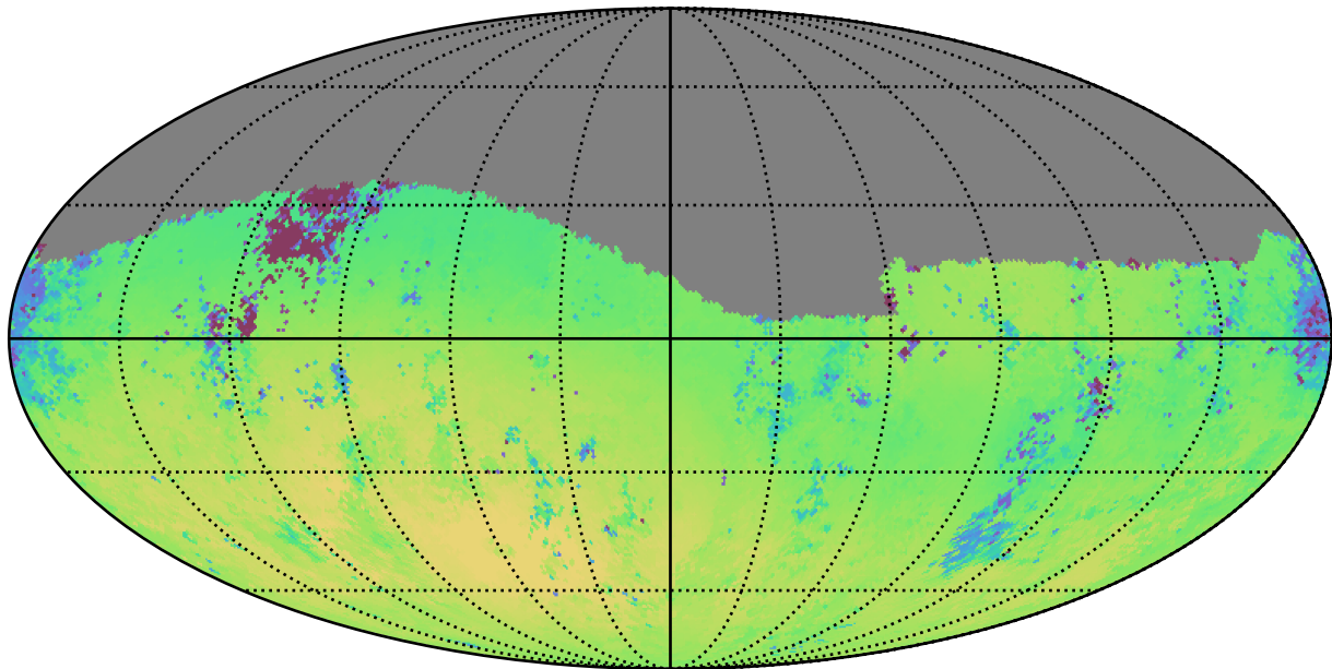
extra_ss_neo4_v3.4_10yrs Yr 1 g band: Median skyBrightness
