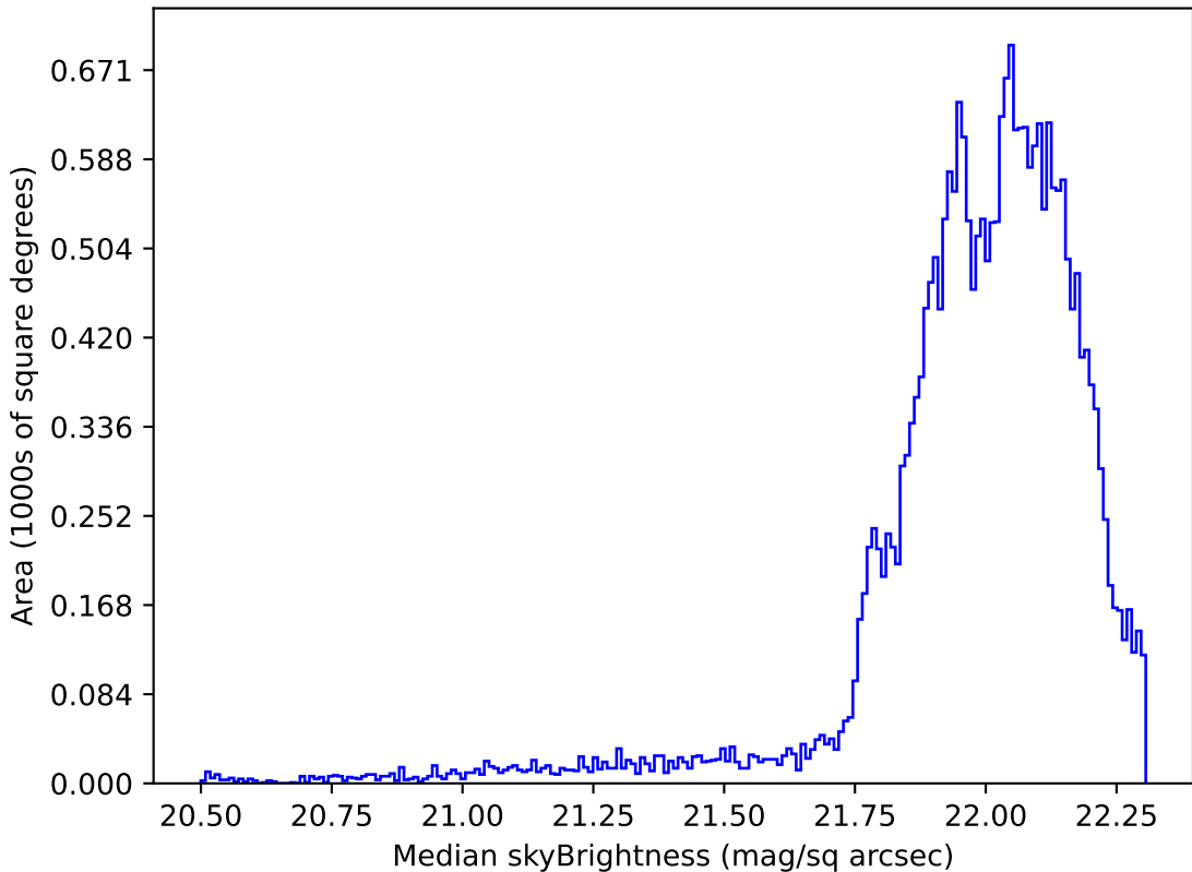
extra_ss_neo4_v3.4_10yrs Yr 1 g band: Median skyBrightness
