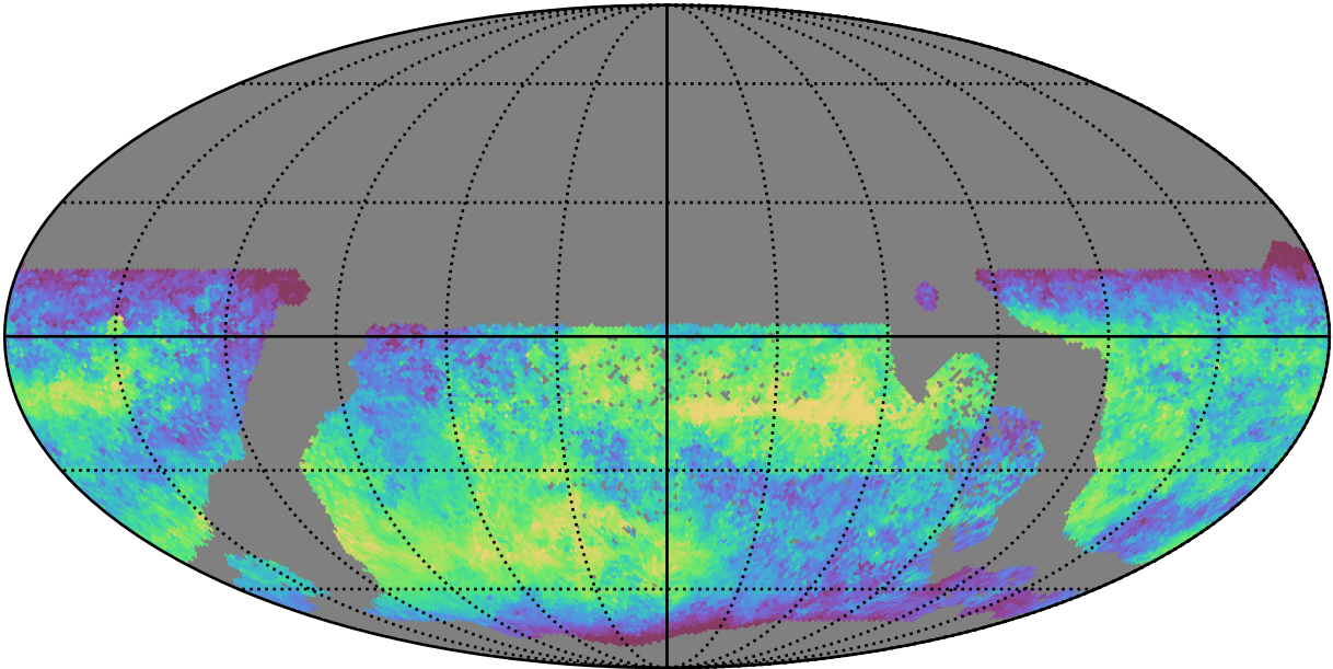
extra_ss_neo4_v3.4_10yrs WFD z band: Median skyBrightness
