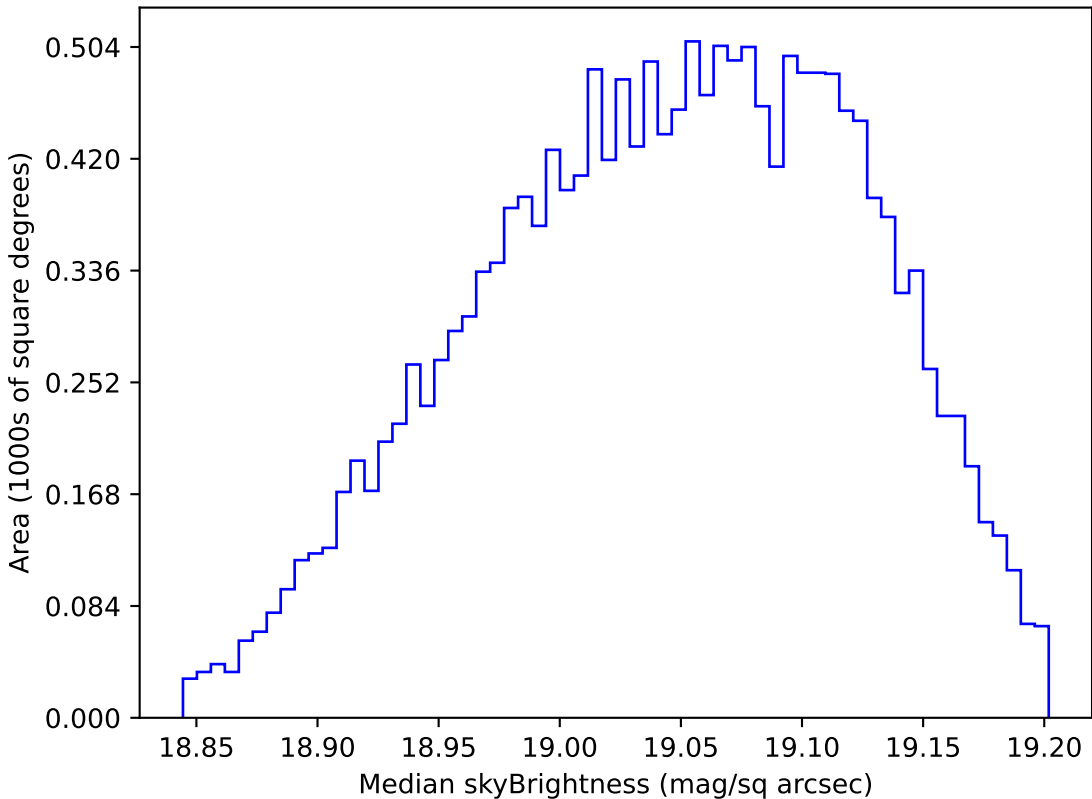
extra_ss_neo4_v3.4_10yrs WFD z band: Median skyBrightness
