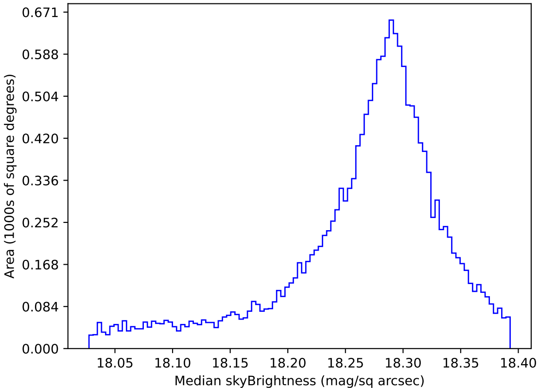
extra_ss_neo4_v3.4_10yrs WFD y band: Median skyBrightness
