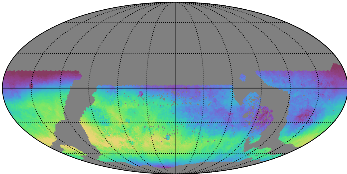
extra_ss_neo4_v3.4_10yrs WFD u band: Median skyBrightness
