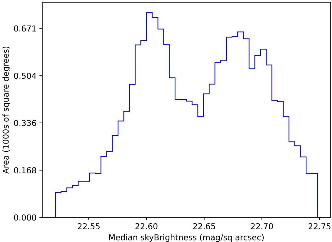
extra_ss_neo4_v3.4_10yrs WFD u band: Median skyBrightness
