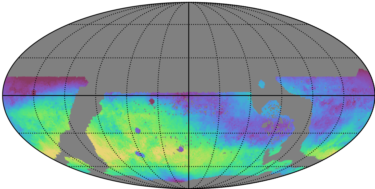
extra_ss_neo4_v3.4_10yrs WFD r band: Median skyBrightness
