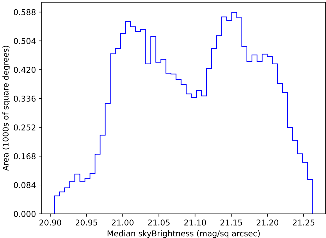
extra_ss_neo4_v3.4_10yrs WFD r band: Median skyBrightness
