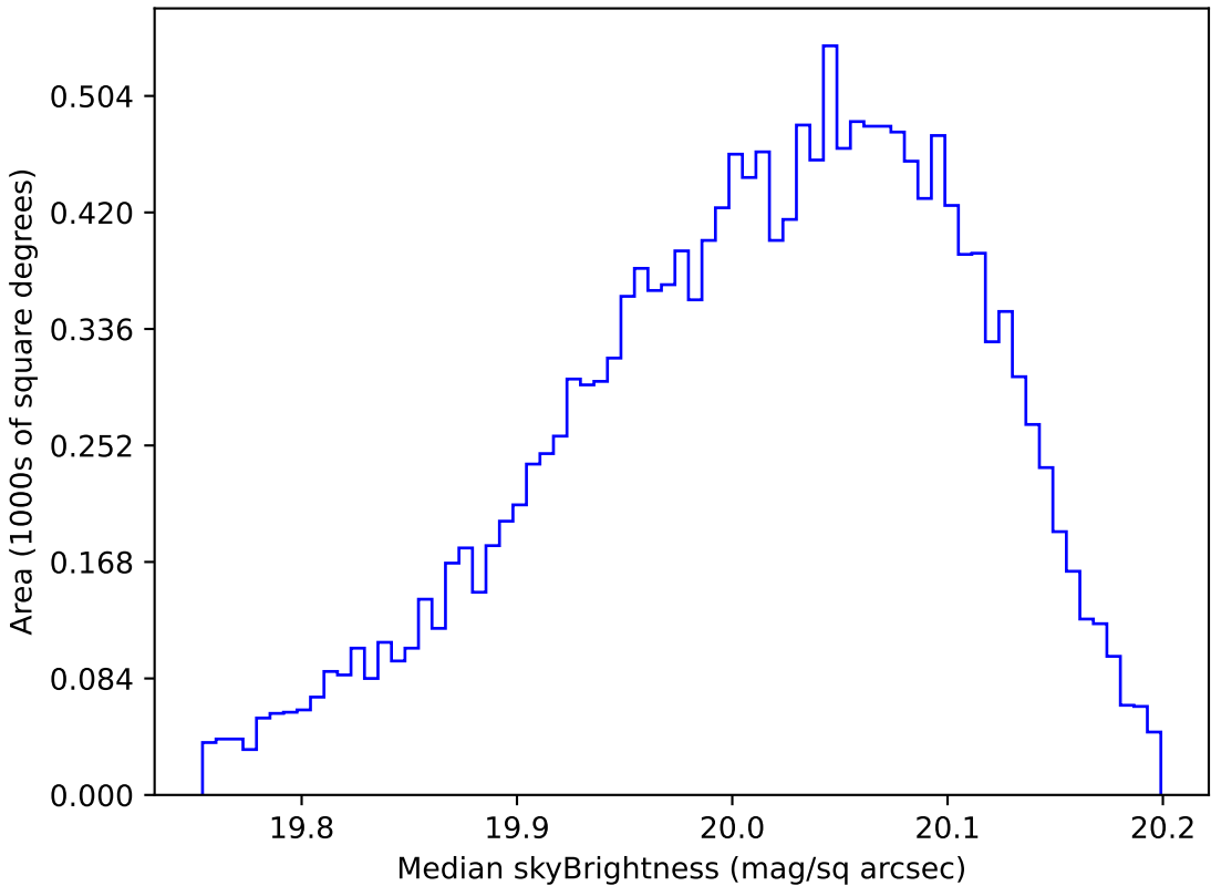
extra_ss_neo4_v3.4_10yrs WFD i band: Median skyBrightness
