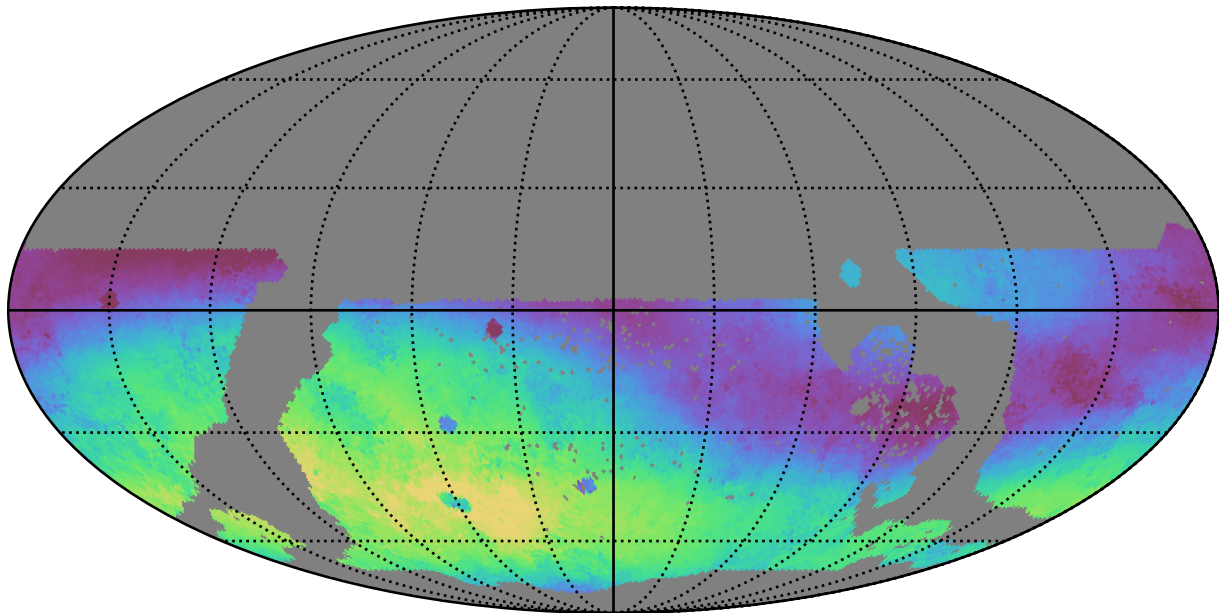
extra_ss_neo4_v3.4_10yrs WFD g band: Median skyBrightness
