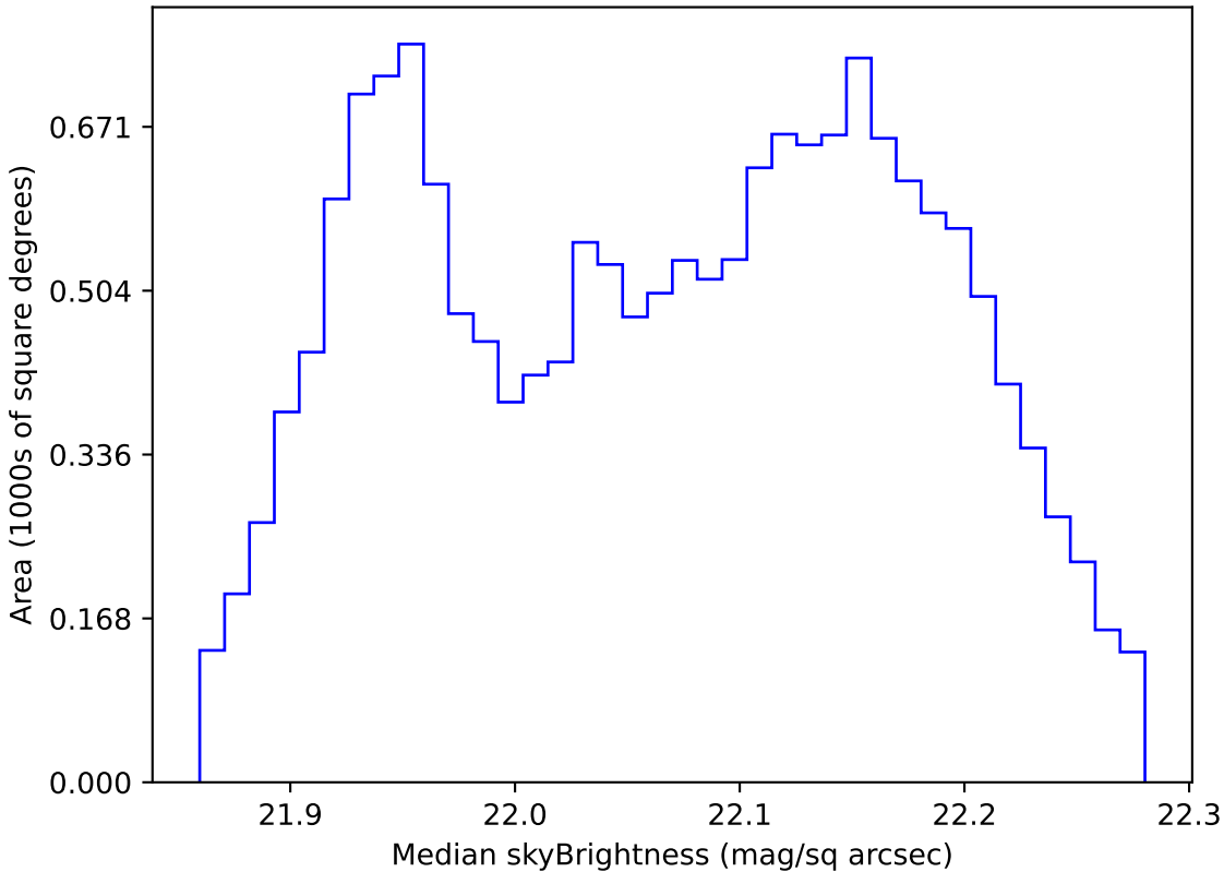
extra_ss_neo4_v3.4_10yrs WFD g band: Median skyBrightness
