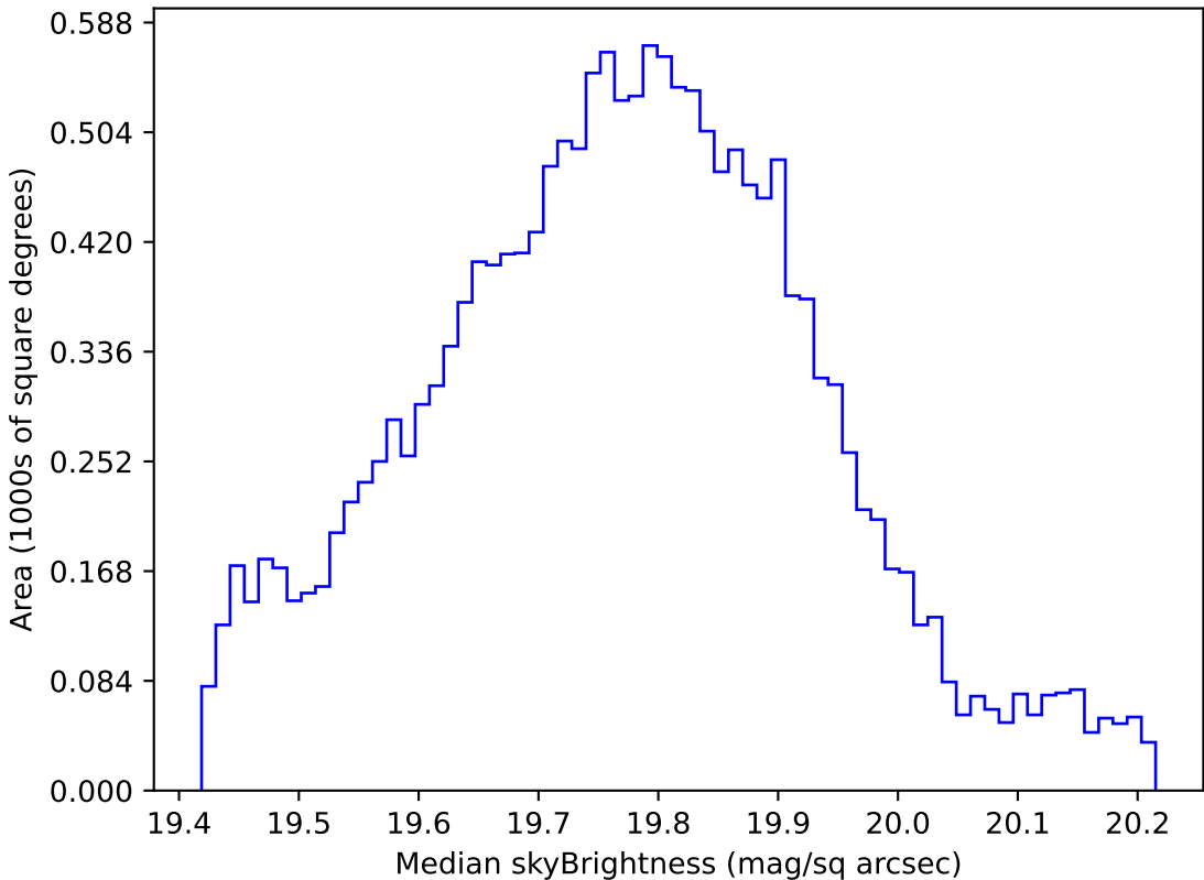
extra_ss_neo4_v3.4_10yrs WFD all bands: Median skyBrightness
