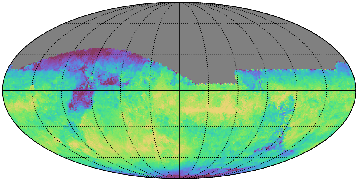
extra_ss_neo4_v3.4_10yrs All sky z band: Median skyBrightness
