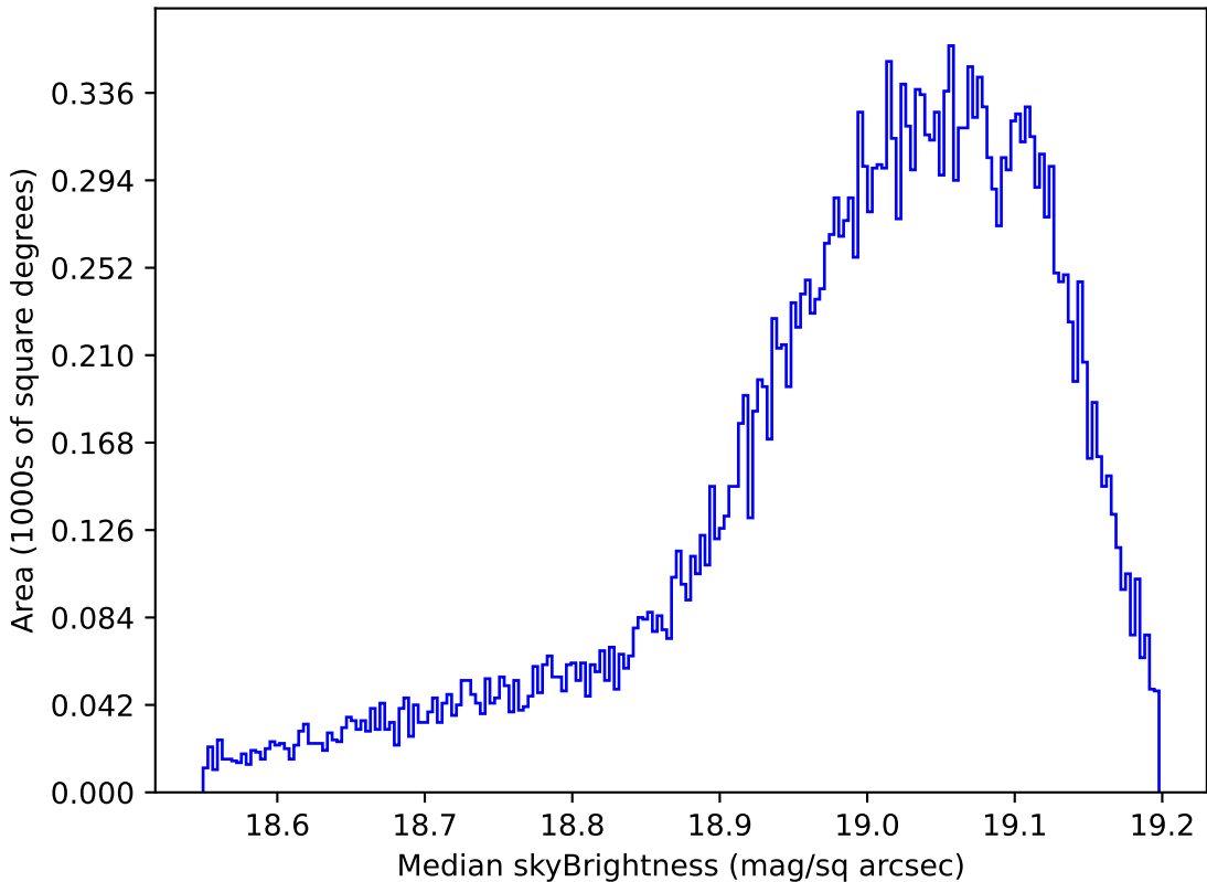
extra_ss_neo4_v3.4_10yrs All sky z band: Median skyBrightness
