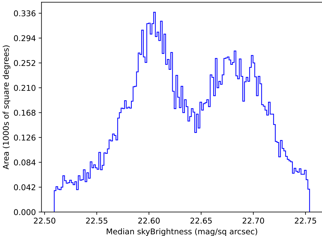
extra_ss_neo4_v3.4_10yrs All sky u band: Median skyBrightness
