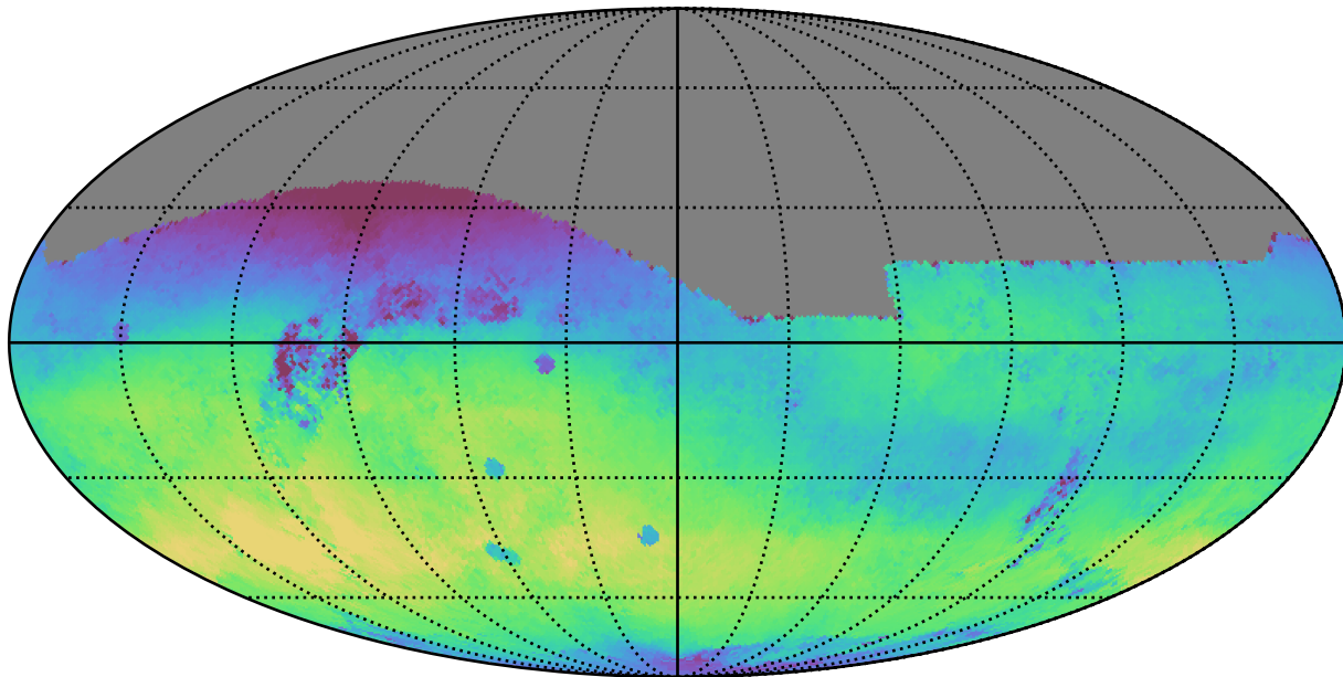
extra_ss_neo4_v3.4_10yrs All sky r band: Median skyBrightness
