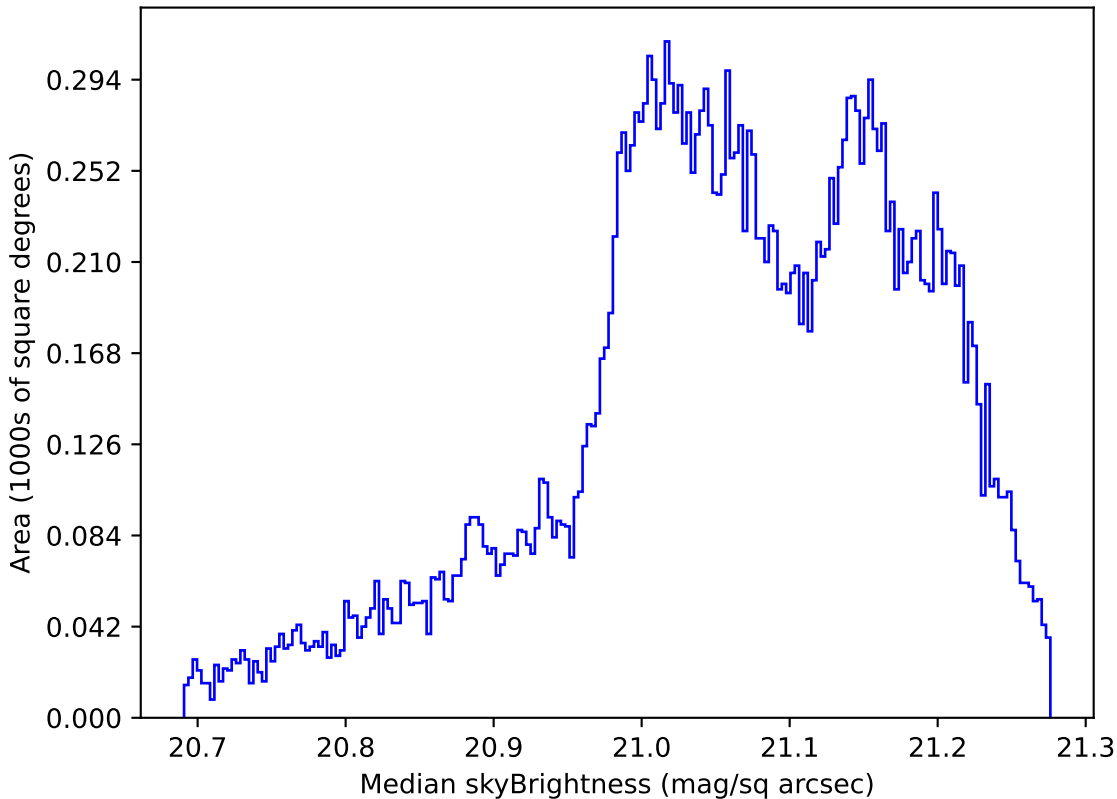
extra_ss_neo4_v3.4_10yrs All sky r band: Median skyBrightness
