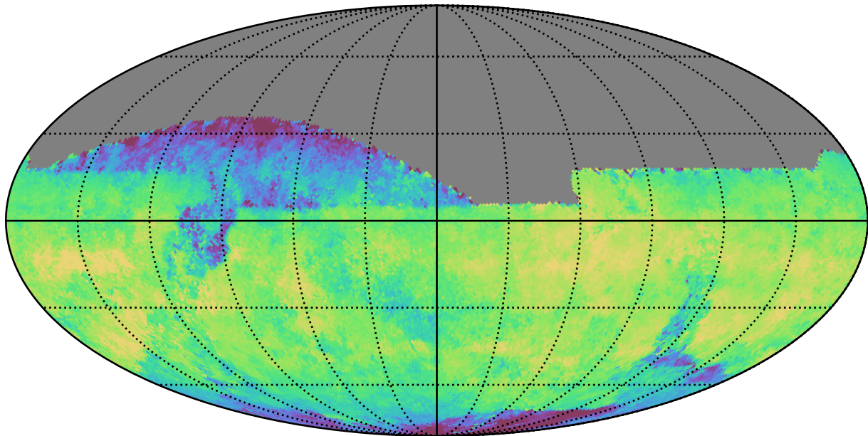
extra_ss_neo4_v3.4_10yrs All sky i band: Median skyBrightness
