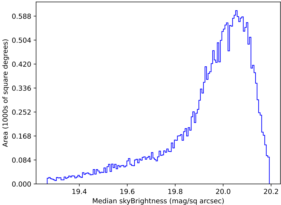
extra_ss_neo4_v3.4_10yrs All sky i band: Median skyBrightness
